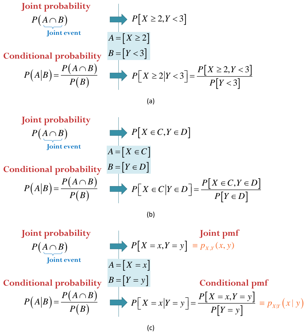
Figure 39: Joints events and conditional probabilities for discrete random variables: (a) an example, (b) the general case, (c) an important special case. Case (c) is used to defined the joint pmf and conditional pmf.
